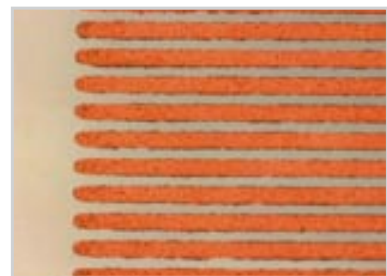
50 µm circuitry before and after repair
