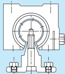
Fig.6 Open type housing
