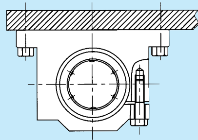
Fig.4 Adjustable type housing
