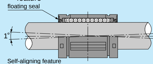
Fig.2 Illustrating floating seal and self-aligning feature
