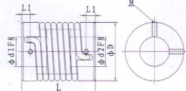
DT SERIES
